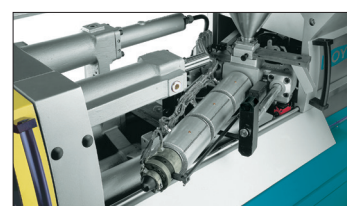
The swivel-out injection unit simplifies the retrofit procedure and maintenance.
